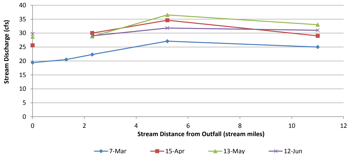
Figure 6 Rock Creek Discharge Measurements Collected by Nebraska DNR 2013
