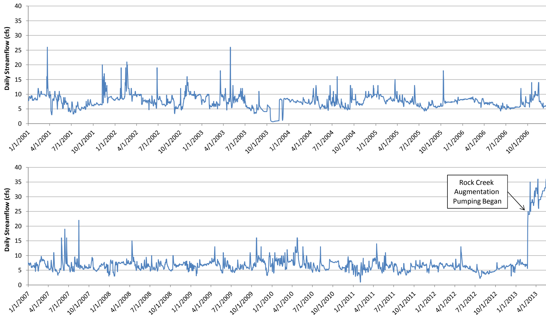
Figure 4 Rock Creek Gage Flow 2001 - May, 2013 Daily cfs
