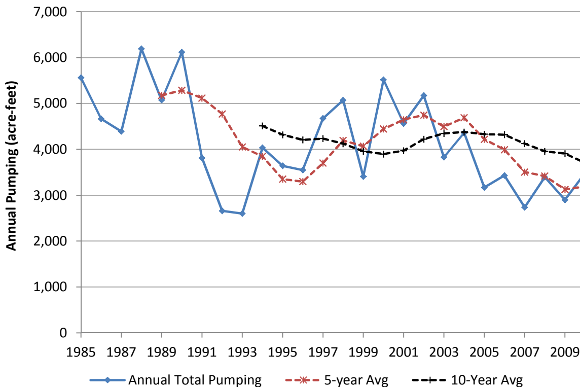
Figure 2 Nebraska Rock Creek Augmentation Project Historical Pumping for Retired Irrigation Wells 1985 - 2010 acre-feet
