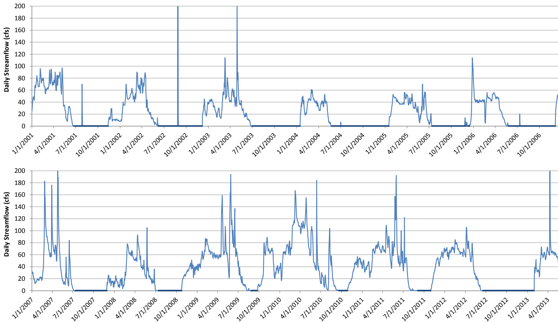
Figure 5 Republican River at Stratton, Nebraska Gage Flow 2001 - May, 2013 Daily cfs
