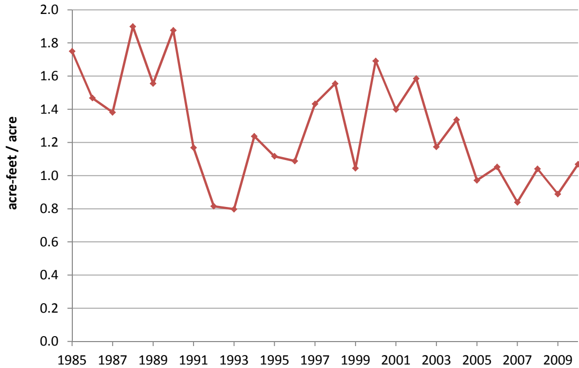
Figure 3 Nebraska Rock Creek Augmentation Project Annual Application Rate for Retired Irrigation Wells 1985 - 2010 acre-feet/acre
